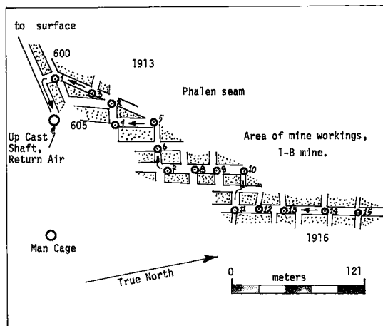
FIG. 4. Part plan of the 1-B mine, #26 Colliery, Glace Bay, N.S. showing numbered sample locations. Elevations (in feet) below sea level. Arrows indicate return air flow (to the surface). Roof-support pillars from mining activity (1913 to 1916) are shown as stippled areas.
