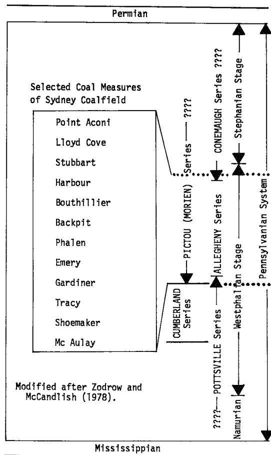
FIG. 1. Coal measures of Sydney coalfield in approximate correlation to the Pennsylvanian series of Nova Scotia (Cumberland to Morien), Pennsylvania (Pottsville to Conemaugh), and Europe (Namurian to Stephanian).
